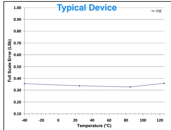
FIGURE 2-27: Full Scale Error (FSE) vs. Temperature.
