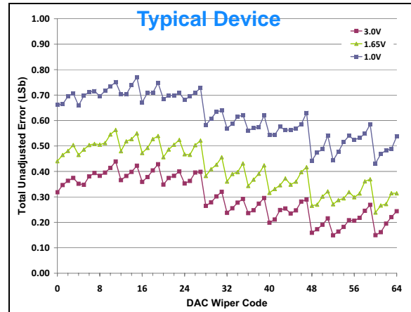
FIGURE 2-77: Total Unadjusted Error vs. Code and V_{REF} V_{DD} = 3.0\text{V} , V_{REF} = 1\text{V} , 1.65\text{V} , and 5.5\text{V} , \text{Temp} = +25^\circ\text{C} .
