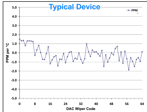
FIGURE 2-60: V_{OUT} Tempco vs. Code \left( \left( \frac{V_{OUT(+125C)} - V_{OUT(-40C)}}{V_{OUT(+25C, Code=FS)}} \right) / 165 \right) * 1,000,000 , V_{DD} = 3.6\text{V} , V_{REF} = 1.65\text{V} .
