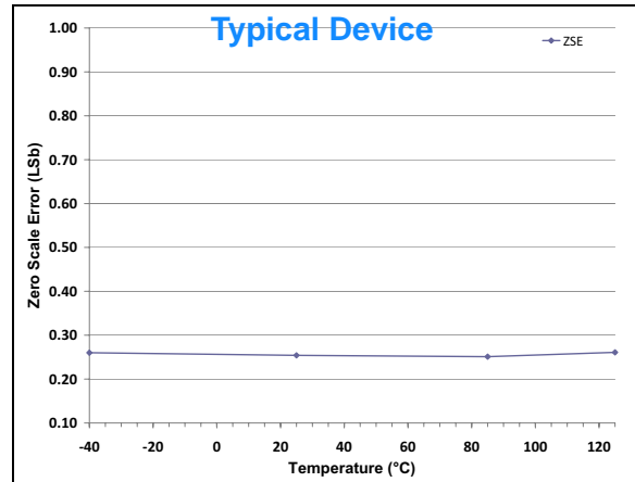
FIGURE 2-37: Zero Scale Error (ZSE) vs. Temperature.
