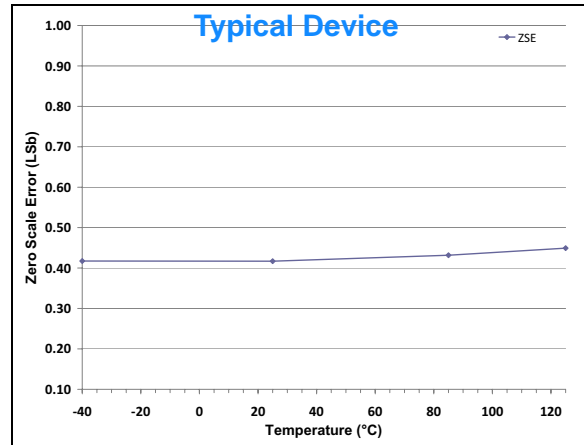
FIGURE 2-38: Zero Scale Error (ZSE) vs. Temperature.
