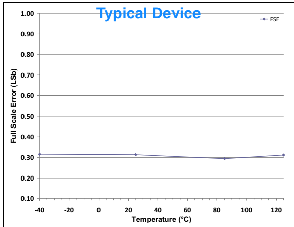
FIGURE 2-30: Full Scale Error (FSE) vs. Temperature.
