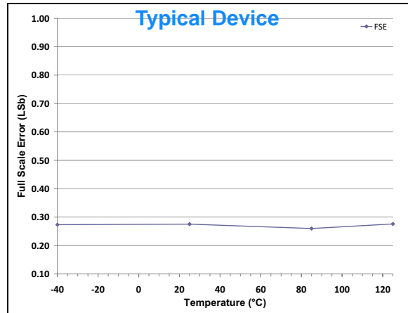
FIGURE 2-32: Full Scale Error (FSE) vs. Temperature.
