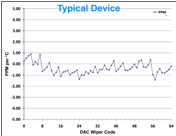
FIGURE 2-56: V_{OUT} Tempco vs. Code \left( \left( \frac{V_{OUT(+125C)} - V_{OUT(-40C)}}{V_{OUT(+25C, Code=FS)}} \right) / 165 \right) * 1,000,000 , V_{DD} = 5.5\text{V} , V_{REF} = 5.5\text{V} .
