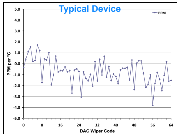
FIGURE 2-61: V_{OUT} Tempco vs. Code \left( \left( \frac{V_{OUT(+125C)} - V_{OUT(-40C)}}{V_{OUT(+25C, Code=FS)}} \right) / 165 \right) * 1,000,000 , V_{DD} = 3.6\text{V} , V_{REF} = 1.0\text{V} .
