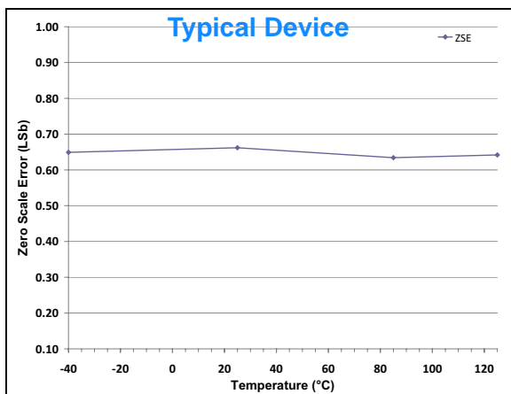
FIGURE 2-42: Zero Scale Error (ZSE) vs. Temperature.
