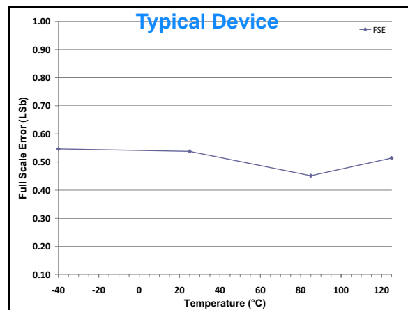
FIGURE 2-28: Full Scale Error (FSE) vs. Temperature.
