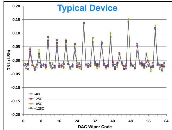
FIGURE 2-15: DNL vs. Code and Temperature. V_{DD} = 3.6\text{V} , V_{REF} = 3.6\text{V}
