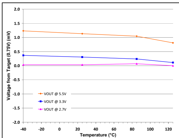
FIGURE 2-85: V_{OUT} Accuracy vs. V_{DD} and Temperature.
