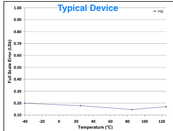
FIGURE 2-26: Full Scale Error (FSE) vs. Temperature.
