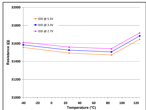
FIGURE 2-88: R_{VREF} Resistances vs. V_{DD} and Temperature.
