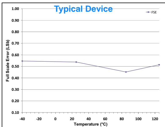
FIGURE 2-31: Full Scale Error (FSE) vs. Temperature.
