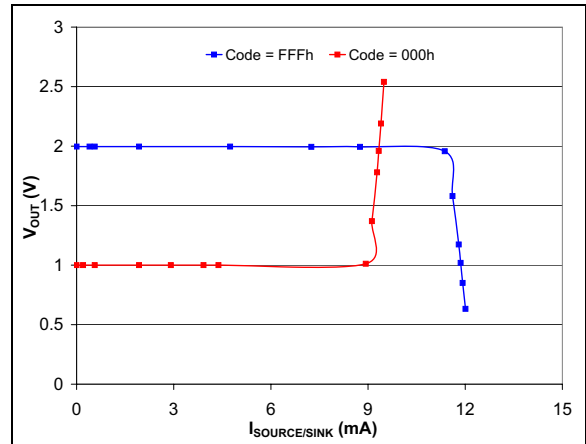
FIGURE 2-86: V_{OUT} vs. Resistive Load. V_{DD} = 3.0\text{V} .
