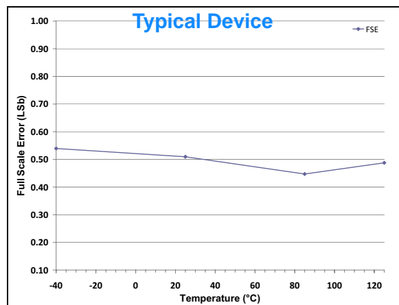
FIGURE 2-33: Full Scale Error (FSE) vs. Temperature.
