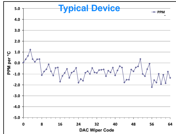
FIGURE 2-59: V_{OUT} Tempco vs. Code \left( \left( \frac{V_{OUT(+125C)} - V_{OUT(-40C)}}{V_{OUT(+25C, Code=FS)}} \right) / 165 \right) * 1,000,000 , V_{DD} = 3.6\text{V} , V_{REF} = 3.6\text{V} .
