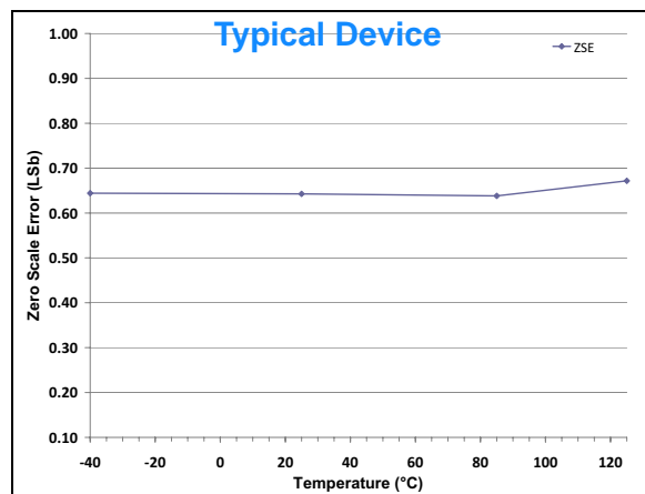
FIGURE 2-44: Zero Scale Error (ZSE) vs. Temperature.
