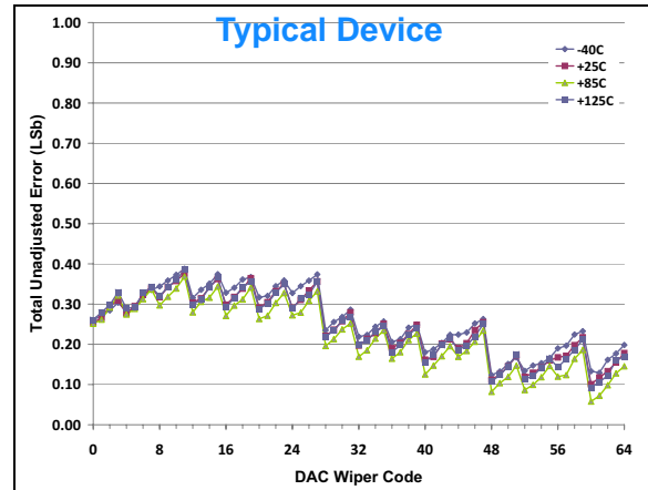
FIGURE 2-48: Total Unadjusted Error vs. Code and Temperature. V_{DD} = 3.6\text{V} , V_{REF} = 3.6\text{V} .
