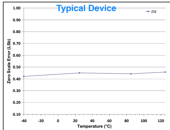
FIGURE 2-43: Zero Scale Error (ZSE) vs. Temperature.
