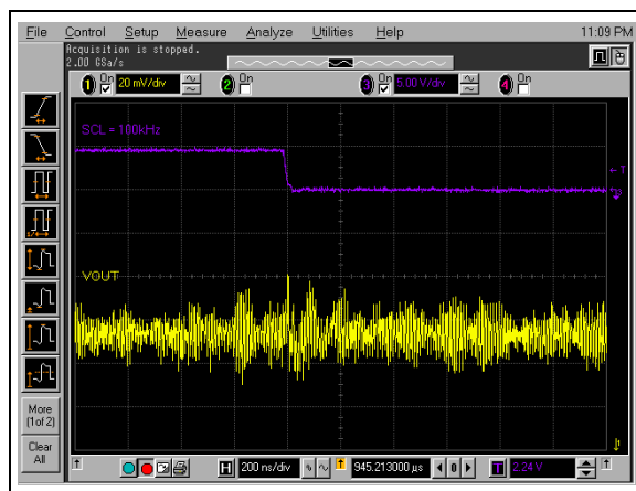
FIGURE 2-93: Digital Feedthrough (SCL signal coupling to V_{OUT} pin); V_{OUT} = 40\text{h} , F_{SCL} = 100\text{kHz} , V_{DD} = 5.0\text{V} , V_{REF} = 5.0\text{V} .
