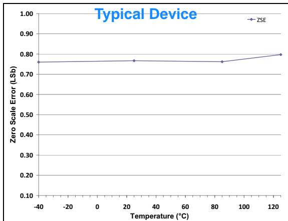
FIGURE 2-36: Zero Scale Error (ZSE) vs. Temperature.
