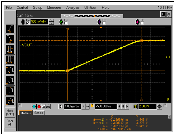
FIGURE 2-89: Zero-Scale to Full-Scale Settling Time (20h to 60h), V_{DD} = 5.0\text{V} , V_{REF} = 5.5\text{V} , R_L = 5\text{k}\Omega , C_L = 1\text{nF} .
