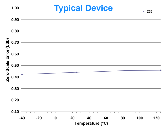
FIGURE 2-41: Zero Scale Error (ZSE) vs. Temperature.
