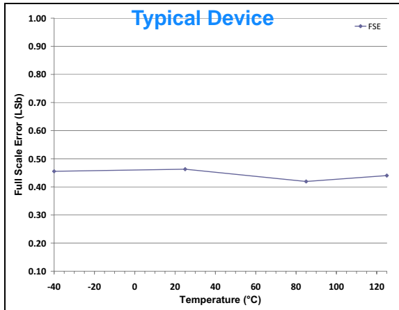
FIGURE 2-24: Full Scale Error (FSE) vs. Temperature.
