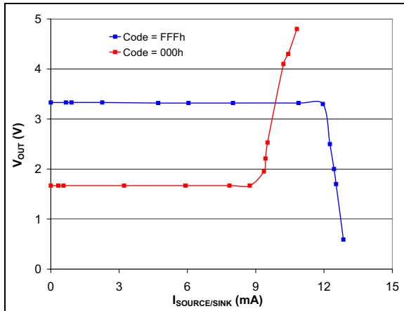
FIGURE 2-83: V_{OUT} vs. Resistive Load. V_{DD} = 5.0\text{V} .
