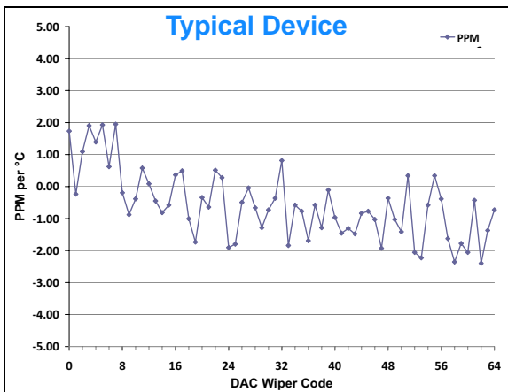
FIGURE 2-58: V_{OUT} Tempco vs. Code \left( \left( \frac{V_{OUT(+125C)} - V_{OUT(-40C)}}{V_{OUT(+25C, Code=FS)}} \right) / 165 \right) * 1,000,000 , V_{DD} = 5.5\text{V} , V_{REF} = 1.0\text{V} .
