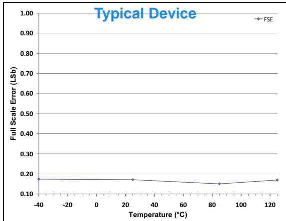
FIGURE 2-23: Full Scale Error (FSE) vs. Temperature.
