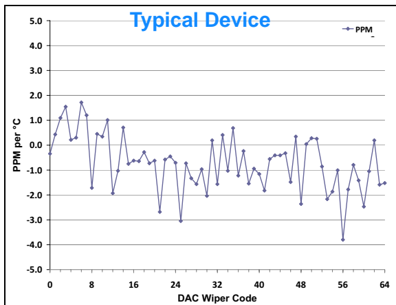
FIGURE 2-64: V_{OUT} Tempco vs. Code \left( \left( \frac{V_{OUT(+125C)} - V_{OUT(-40C)}}{V_{OUT(+25C, Code=FS)}} \right) / 165 \right) * 1,000,000 , V_{DD} = 3.0\text{V} , V_{REF} = 1.0\text{V} .
