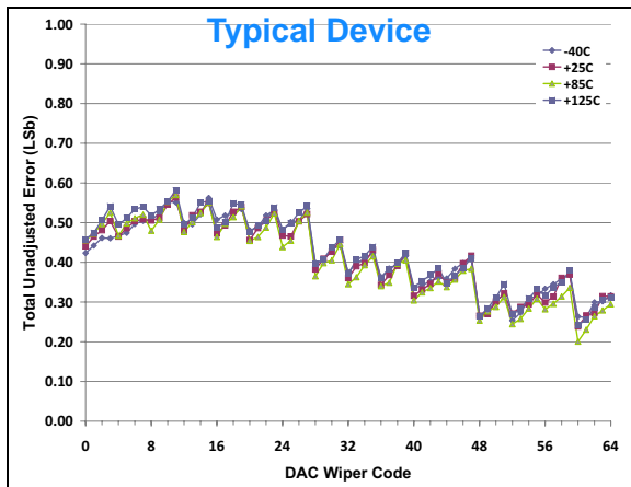
FIGURE 2-52: Total Unadjusted Error vs. Code and Temperature. V_{DD} = 3.0\text{V} , V_{REF} = 1.65\text{V} .
