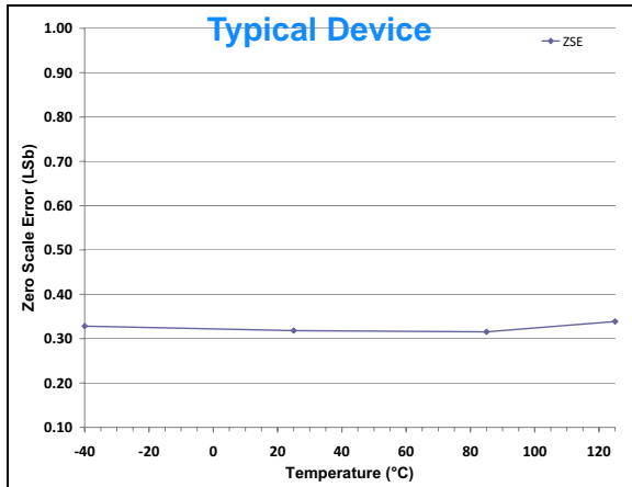
FIGURE 2-40: Zero Scale Error (ZSE) vs. Temperature.
