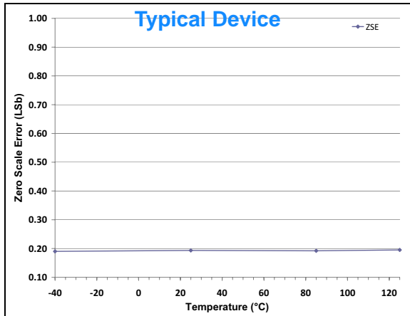
FIGURE 2-34: Zero Scale Error (ZSE) vs. Temperature.
