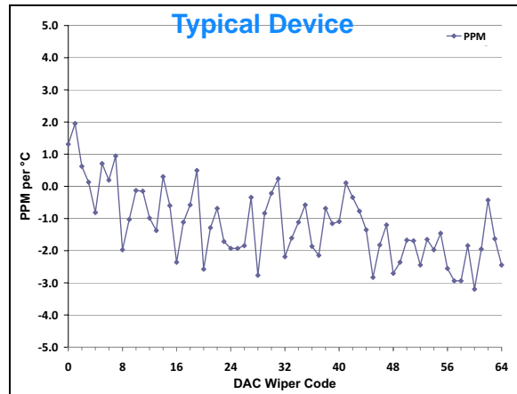
FIGURE 2-66: V_{OUT} Tempco vs. Code \left( \left( \frac{V_{OUT(+125C)} - V_{OUT(-40C)}}{V_{OUT(+25C, Code=FS)}} \right) / 165 \right) * 1,000,000 , V_{DD} = 2.7\text{V} , V_{REF} = 1.0\text{V} .
