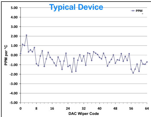
FIGURE 2-57: V_{OUT} Tempco vs. Code \left( \left( \frac{V_{OUT(+125C)} - V_{OUT(-40C)}}{V_{OUT(+25C, Code=FS)}} \right) / 165 \right) * 1,000,000 , V_{DD} = 5.5\text{V} , V_{REF} = 1.65\text{V} .
