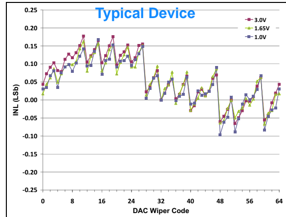
FIGURE 2-69: INL vs. Code and V_{REF} V_{DD} = 3.0\text{V} , V_{REF} = 1\text{V} , 1.65\text{V} , and 5.5\text{V} , \text{Temp} = +25^\circ\text{C} .
