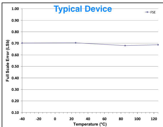
FIGURE 2-25: Full Scale Error (FSE) vs. Temperature.
