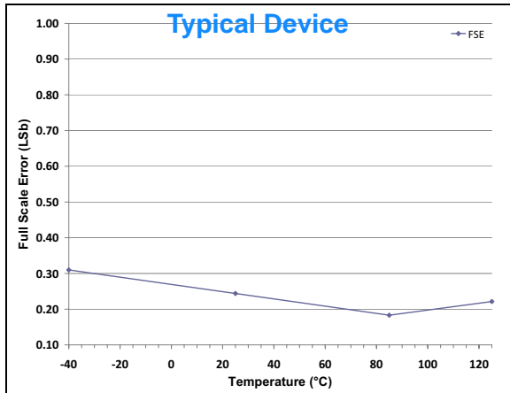
FIGURE 2-29: Full Scale Error (FSE) vs. Temperature.
